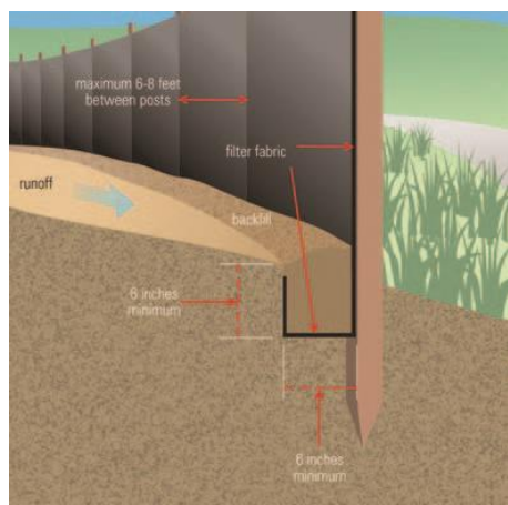
Illustration of a proper silt fence installation.
